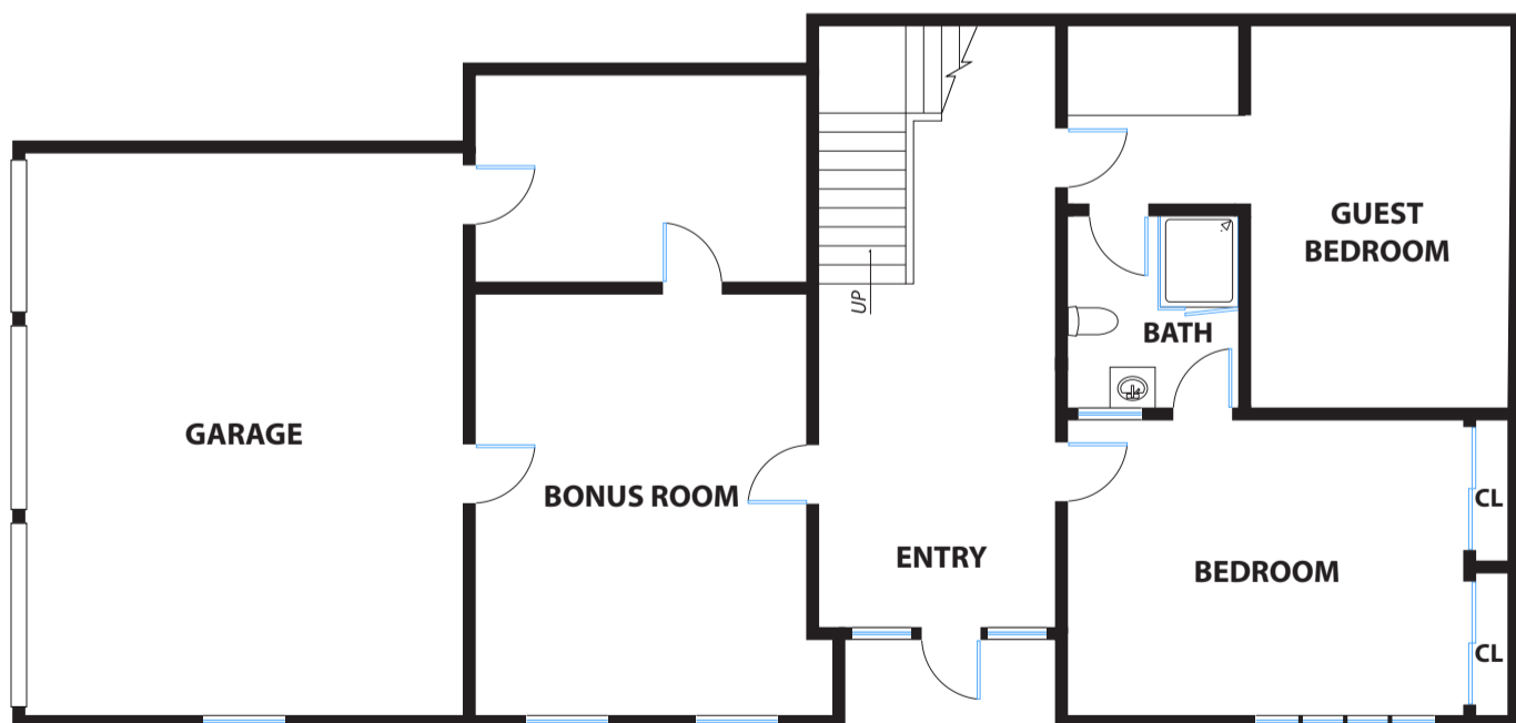
FIRST FLOOR
